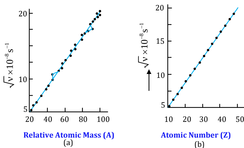
Moseley's Experiment
