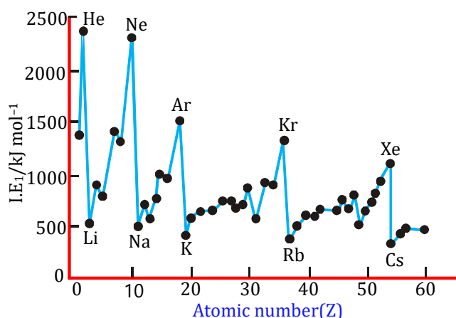
Variation of first ionization energy ( I.E. ) 1 with atomic number for elements with Z = 1 to 60
