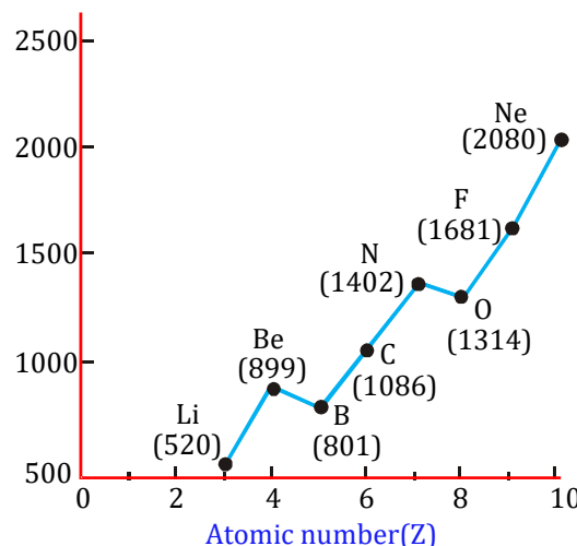
First ionization energy ( I.E. ) 1 of elements of the second period as a function of atomic number ( Z )
